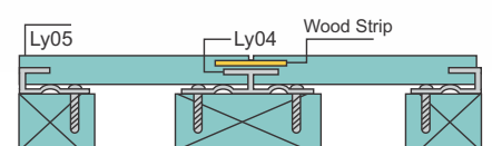
Cross-section Structure
